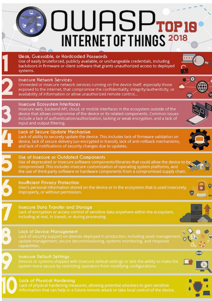
OWASP IOT TOP10 2018
